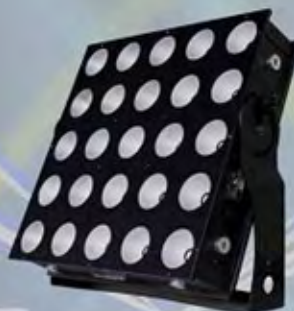
Pixel Matrix
